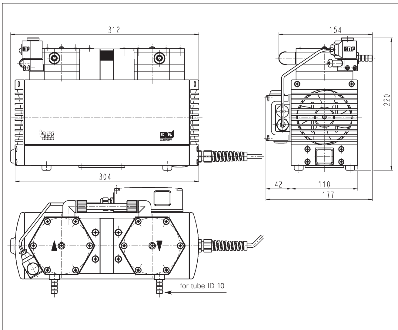
Dimensions (mm)
