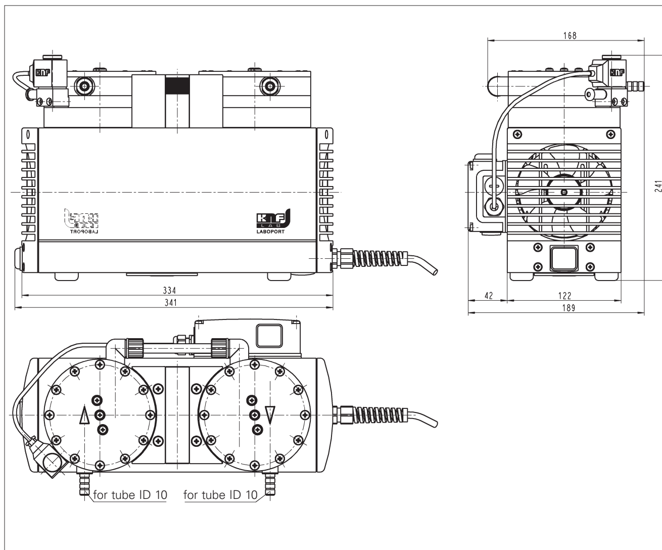
Dimensions (mm)
